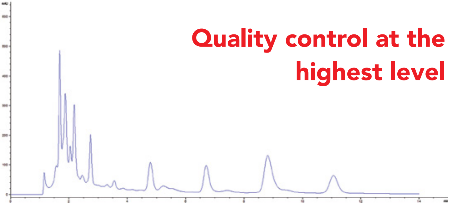
Cordyceps and adenosine evaluation by HPLC
